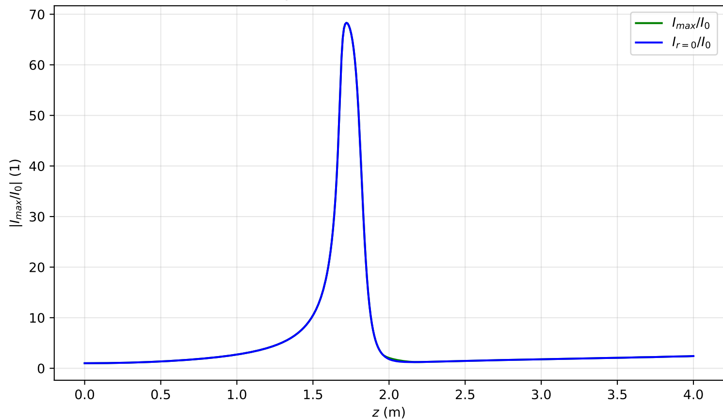
I_{max}(x = 0, y = 0, z)/I_0 , Pin=1.5P_{cr} , artificial time
